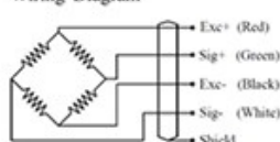
Wiring Diagram
